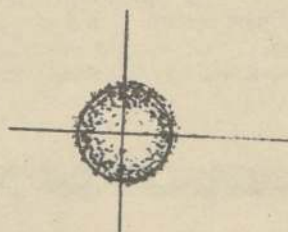
Orbital "s"
