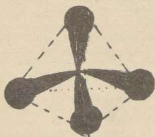
Diagrama orbital
