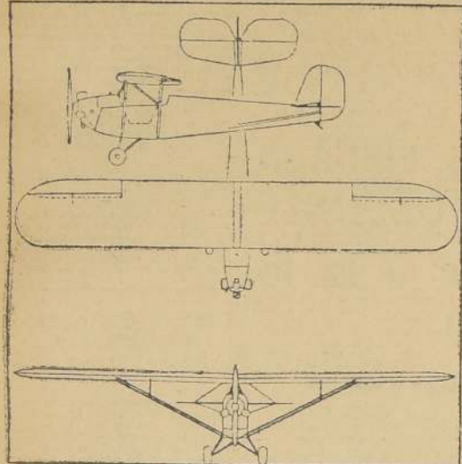
AMERICAN EAGLE (EAGLE). — MONOPLANO DE ALA ALTA
