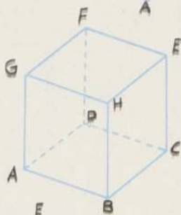
HEXAEDRO REGULAR (Cubo)
